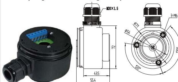
TL-BM(magnetic mounting base)
